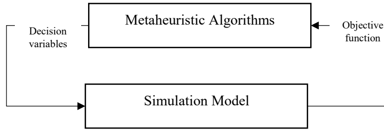
Figure 6. Simulation-Optimization Approach
